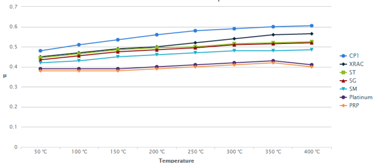
Friction Performance VS Temperature
